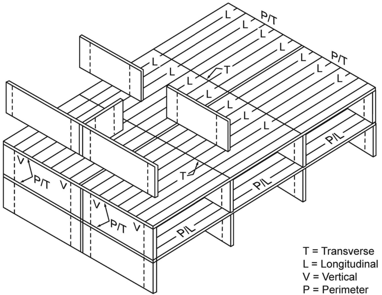
GURE 1614.4 LONGITUDINAL, PERIMETER, TRANSVERSE AND VERTICAL TIES
