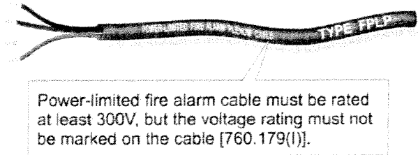
Listing and Marking of Type PLFA Cable - Rating 760.179(C)
