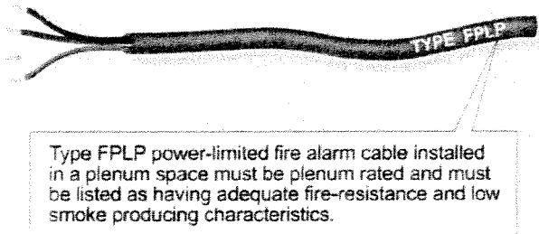
Listing and Marking of PLFA Cable - Type FPLP 760.179(D)
